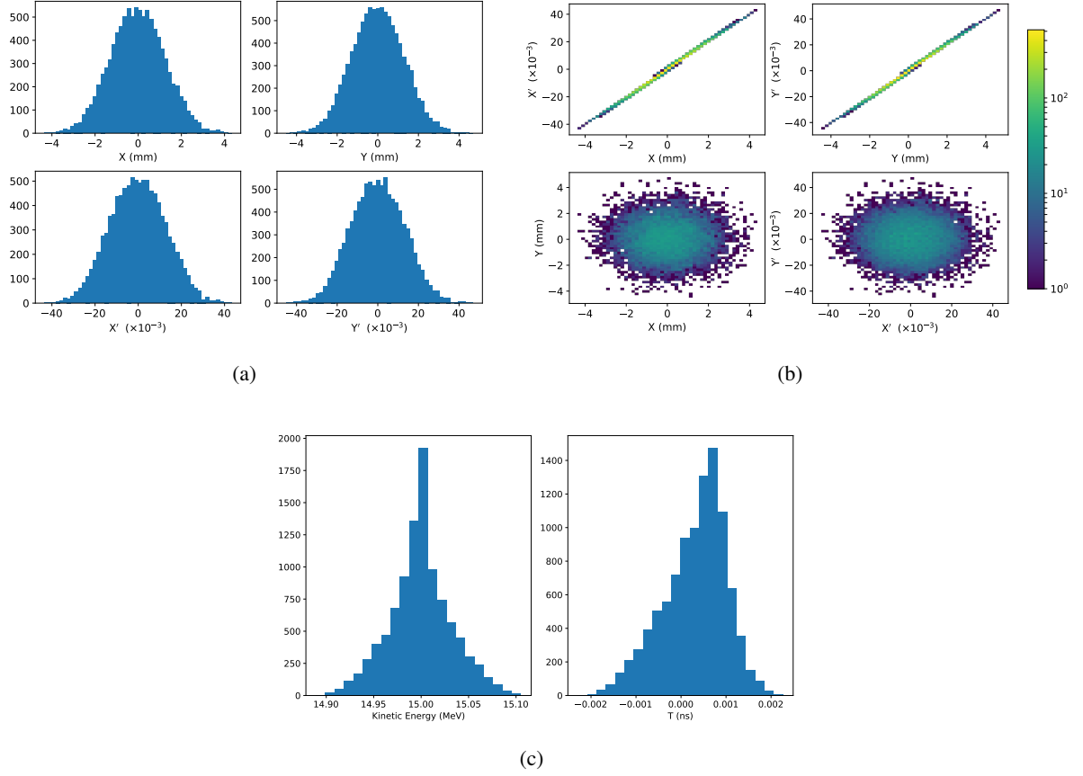
Figure 10: Beam phase space distributions in the transverse plane, (X, Y) ; X' and Y' give the slope relative to the Z axis. The transverse phase space is shown in figures a and b. The longitudinal phase space, kinetic energy and time, T , is shown in c. The phase-space distributions are plotted 10 cm from the laser target.
