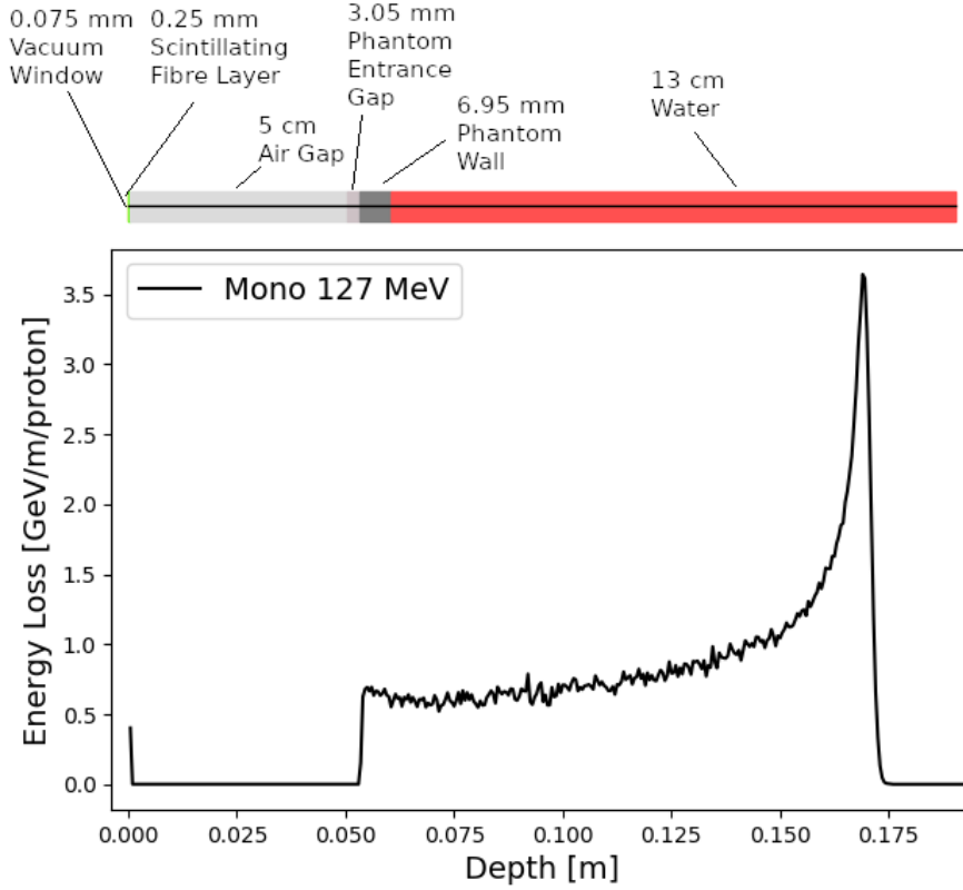
Figure 39: Simulation of the expected range in a water phantom for a 127 MeV proton beam.
