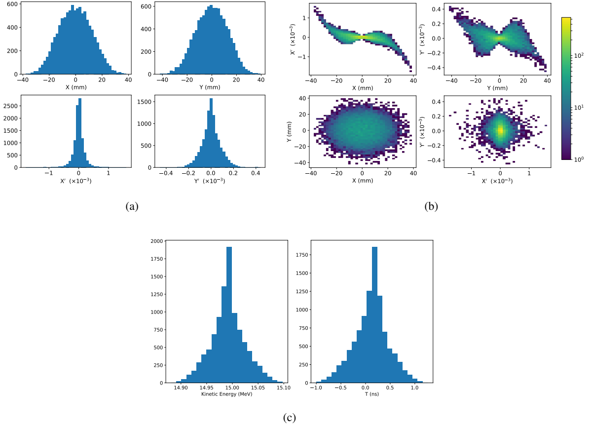
Figure 12: Beam phase space distributions in the transverse plane, (X, Y) ; X' and Y' give the slope relative to the Z axis. The transverse phase space is shown in figures a and b. The longitudinal phase space, kinetic energy and time, T , is shown in c. The phase-space distributions are plotted at the in-vitro end station without octupolar focusing.
