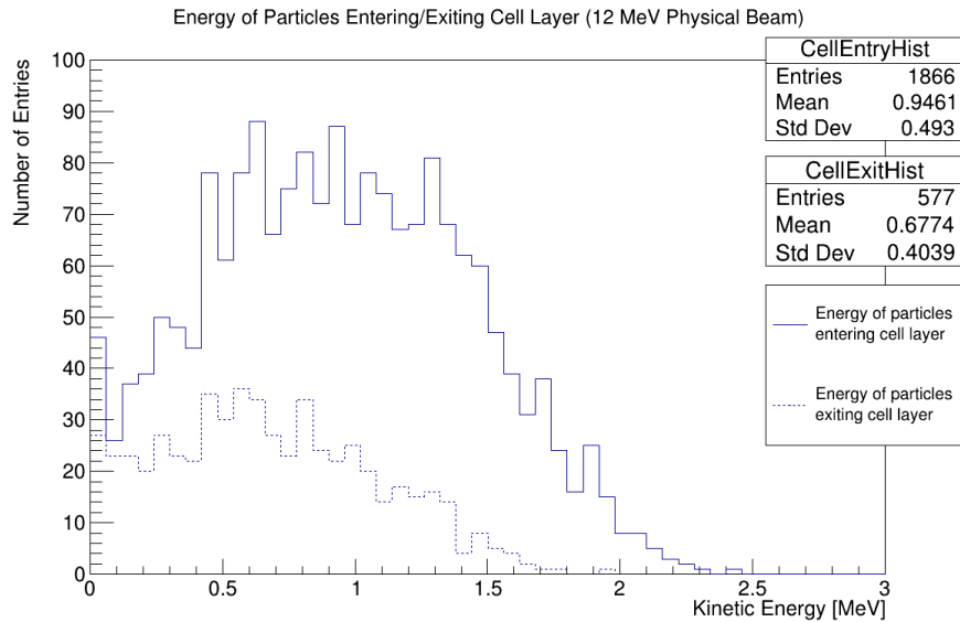
Figure 24: Simulation results of the energy distribution of particles entering and exiting the cell layer for a physical 12 MeV beam.
