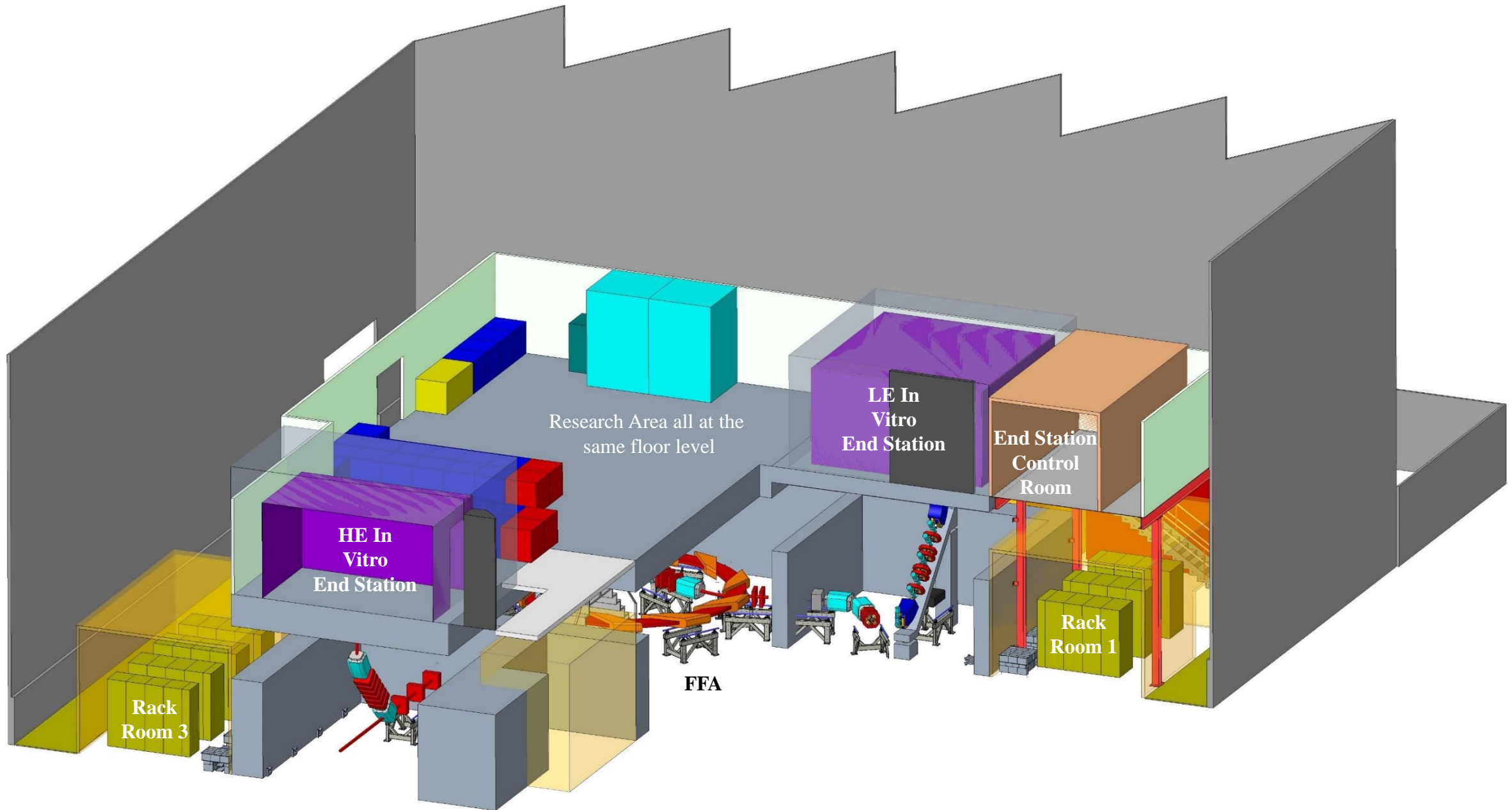
Figure #: Cross section isometric through building
