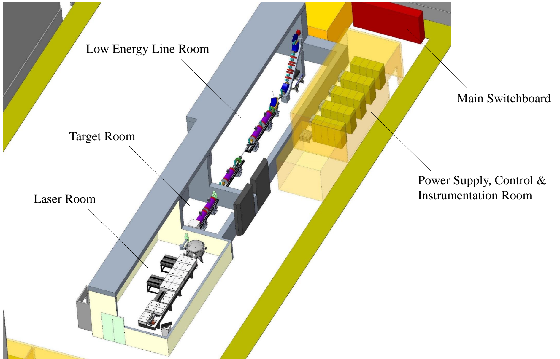
Figure #: Stage 1 Building concept with room cutaway at larger scale
