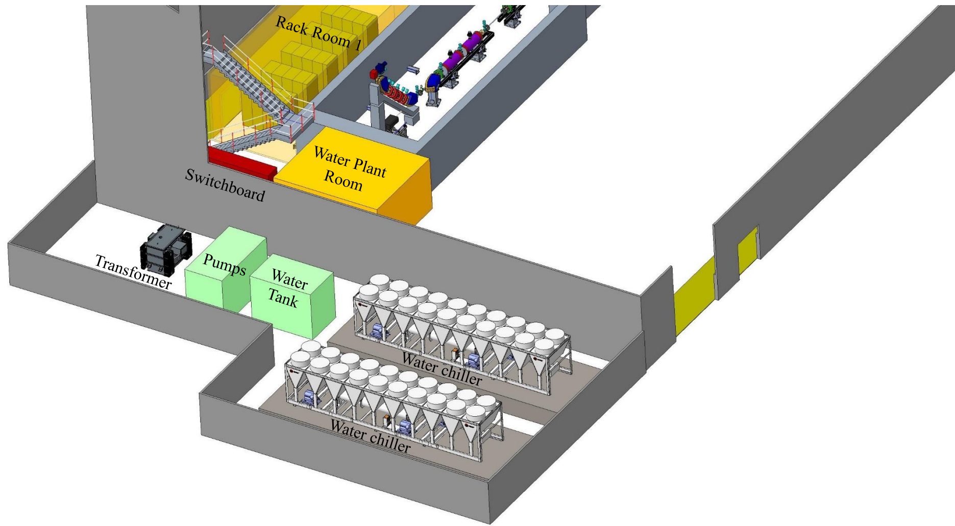
Figure #: Water chillers and Transformer pen
