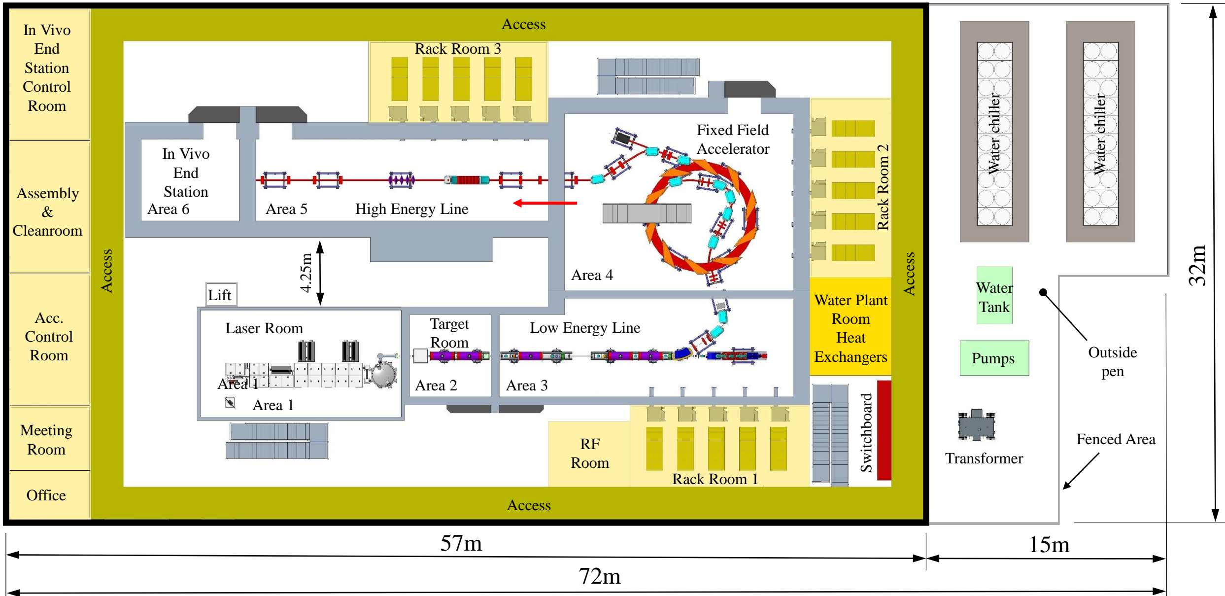
Figure #: Plan View Layout of Facility – Stage 1 & 2
