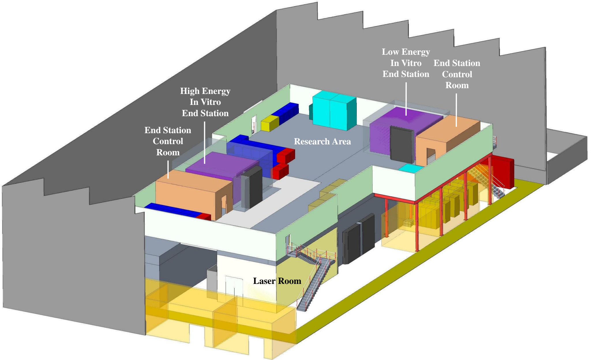
Figure #: Building Concept Design
