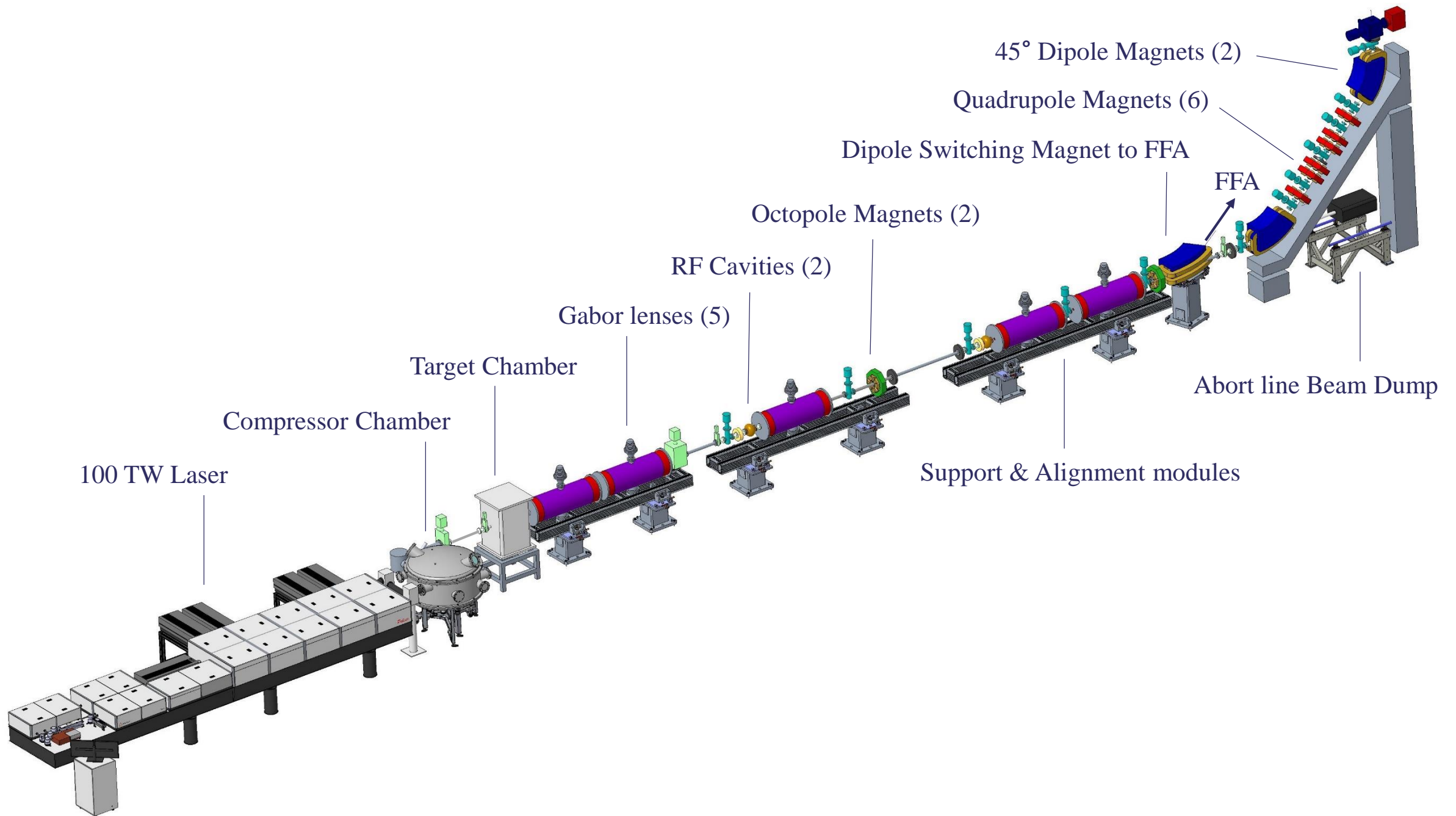
Figure #: Stage 1 Engineering Concept Design
