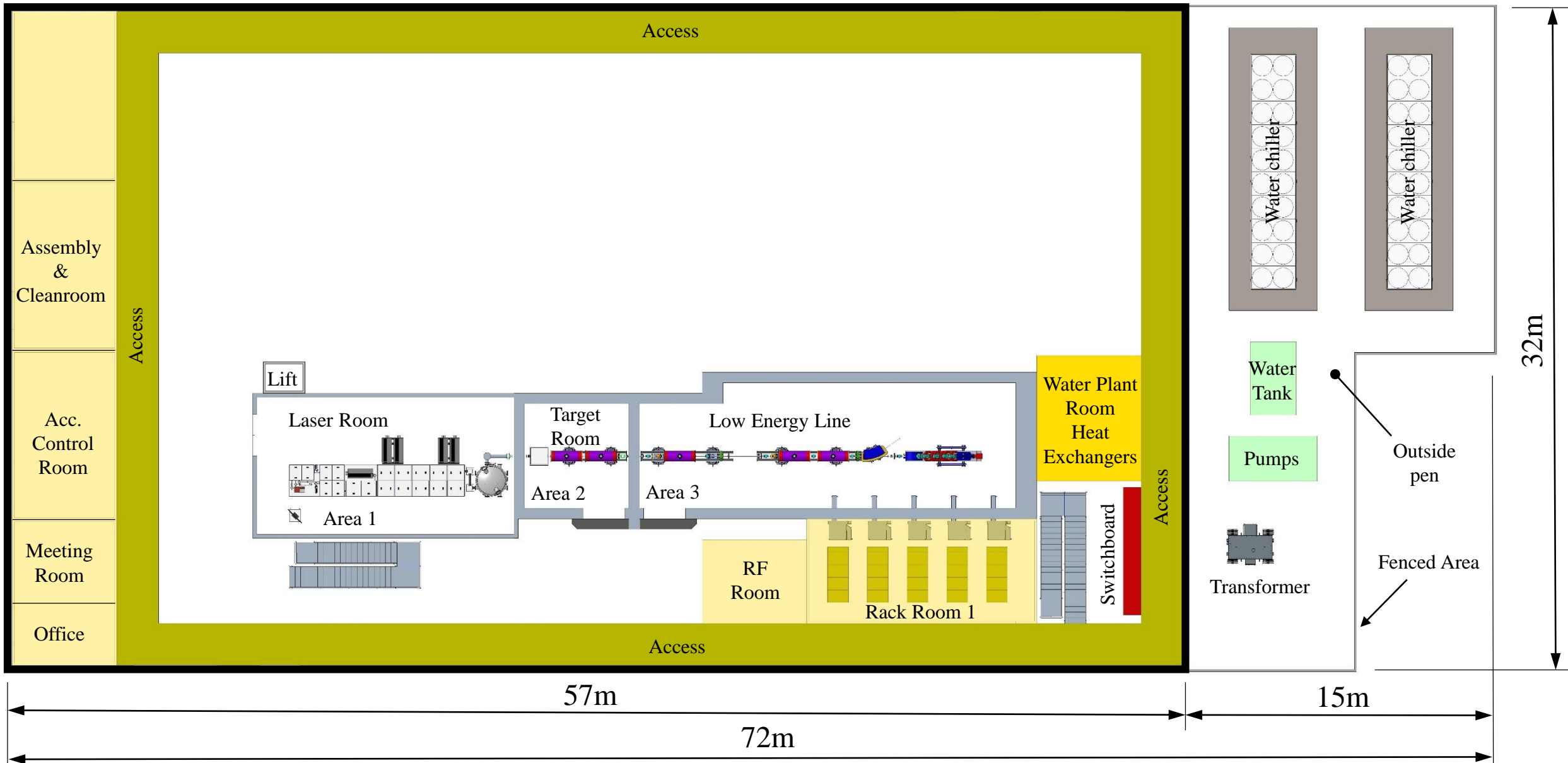
Figure #: Plan View Layout of Facility – Stage 1
