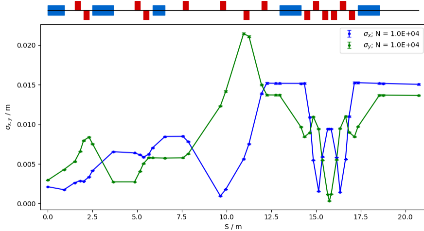
Figure 37: BDSIM simulation for a 127 MeV proton beam from the start of the extraction line to the in vitro end station where the extraction line quadrupoles are set to provide a matched beam with \beta_{x,y} = 58 at the beginning of the arc. The plot shows the evolution of RMS beam size (in x and y) as a function of position along the beam line.
