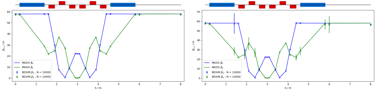
Figure 35: Comparison of MAD-X and BDSIM simulation of 15 MeV (left) and 127 MeV (right) proton beam passing through the high energy in vitro arc simulated with 10^4 particles.
