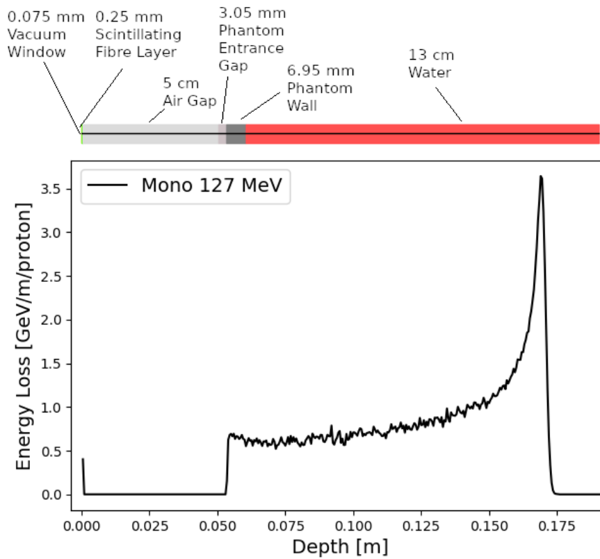
Figure 38: Simulation of the expected range in a water phantom for a 127 MeV proton beam.
