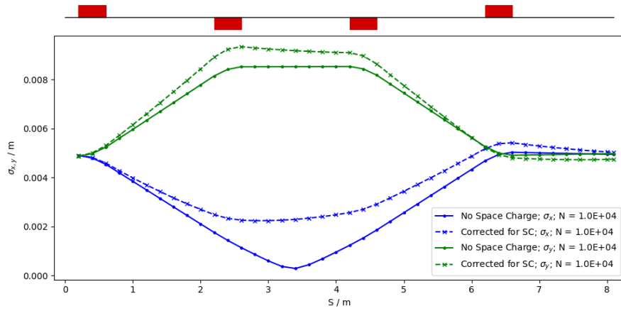
Figure 43: GPT simulations of the in vivo beamline for a 15 MeV proton beam with quadrupoles adjusted to compensate for the effects of space charge. The solid lines are from the simulation with space charge turned off, the dashed lines are with space charge turned on and with modified quadrupole settings.
