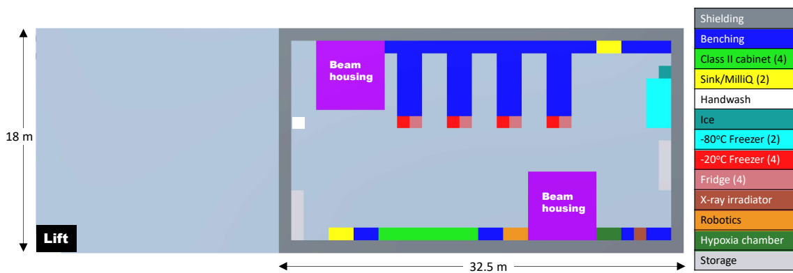
Figure 54: Top-down view of the floor layout of the in vitro end stations level.
