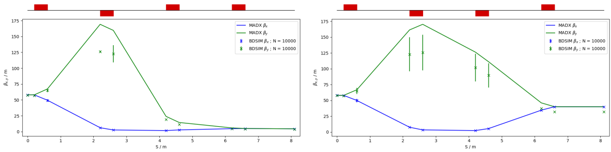
Figure 45: MAD-X and BDSIM comparison simulations of the in vivo beamline for a 127 MeV proton beam with quadrupoles matched to \beta_{x,y} = 4.5 (left) and \beta_{x,y} = 40 (right) for 10^4 particles.
