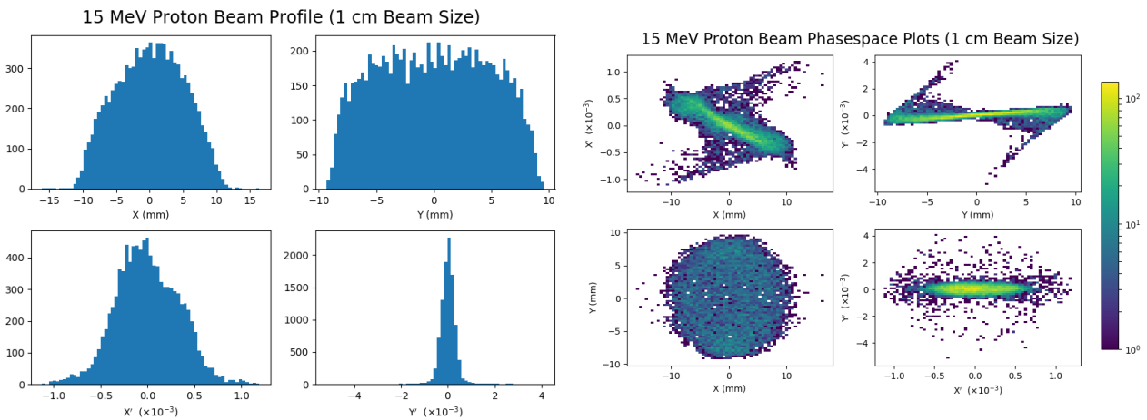
Figure 44: GPT simulations of beam profile and phase plots of a 15 MeV proton beam with the effects of space charge compensated for.
