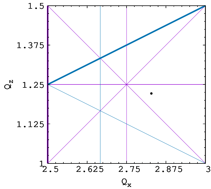
Figure 30: The working point of the FFA ring on the tune diagram.
