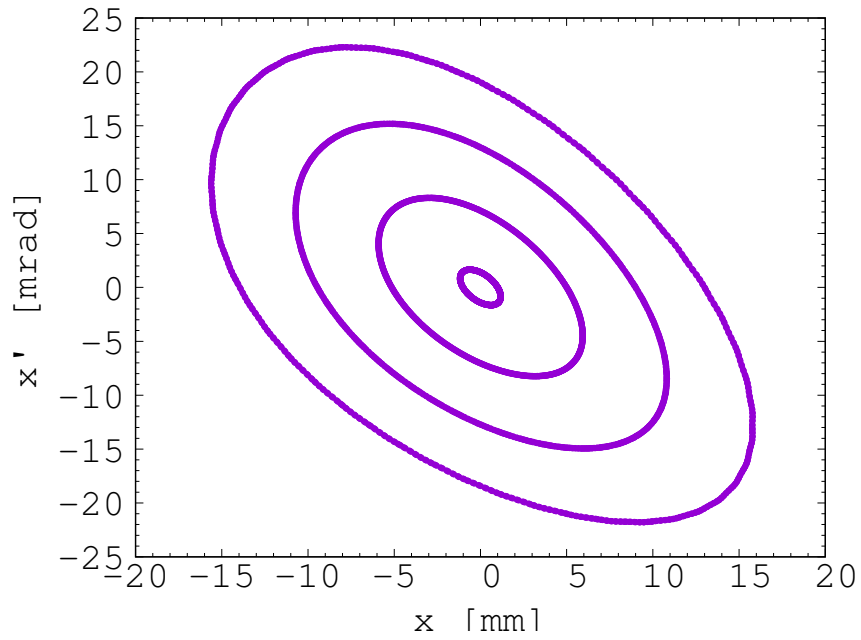
Figure 32: The results of the horizontal dynamical acceptance study in the FFA ring. The 1 mm offset is assumed in the vertical plane.
