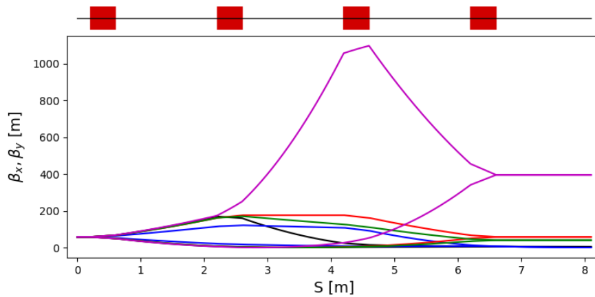
Figure 40: \beta_x and \beta_y functions for the in vivo beam line matching from \beta_{x,y} = 58 to \beta_{x,y} = 395 (magenta), \beta_{x,y} = 58 (red), \beta_{x,y} = 40 (green), \beta_{x,y} = 4.5 (black) and \beta_{x,y} = 0.347 (blue).
