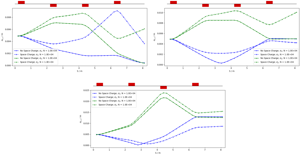
Figure 42: GPT simulations of the in vivo beamline for a 15 MeV proton beam with quadrupoles matched to \beta_{x,y} = 0.347 (upper left), \beta_{x,y} = 58 (upper right) and \beta_{x,y} = 395 (bottom) for 10^4 particles to investigate the effects of space charge. The solid line is when space charge is turned off, the dashed line when space charge is turned on.
