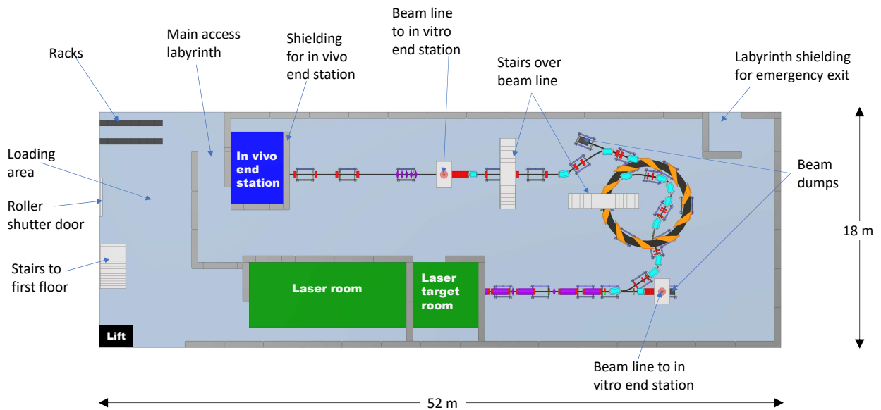
Figure 53: Top-down view of the floor layout of the accelerator level.
