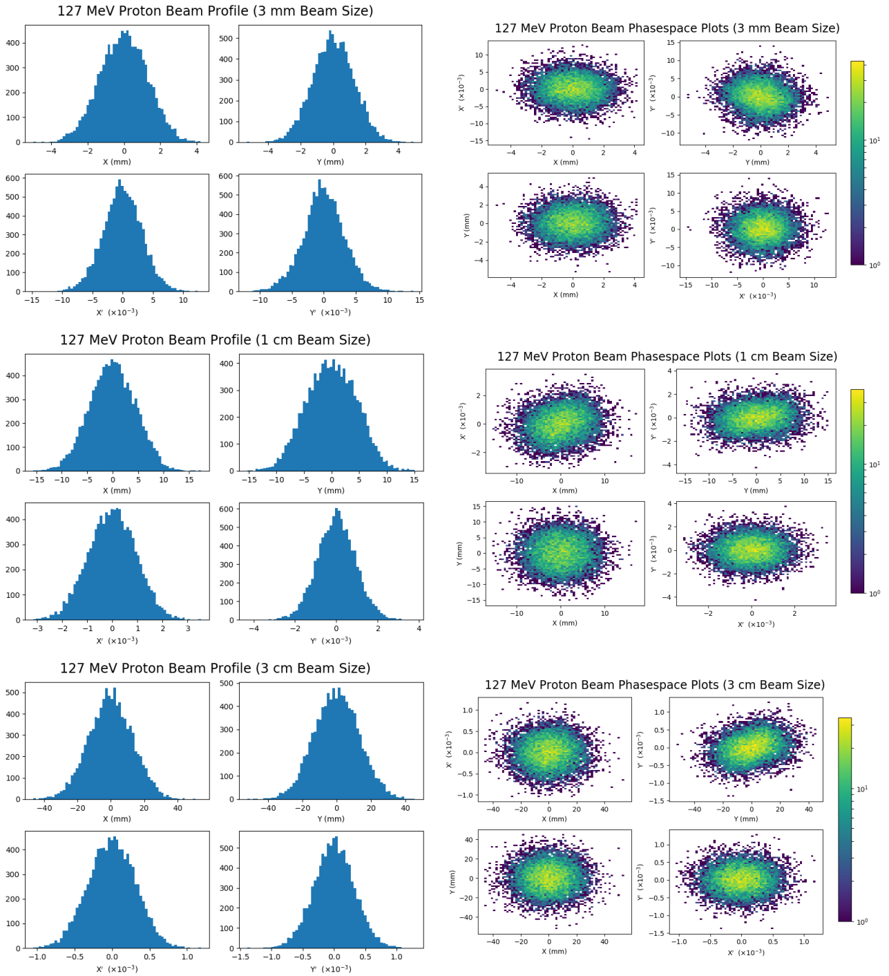
Figure 47: Beam profile and phase space plots in the end station for 127 MeV proton beam from GPT simulations with space charge on. Top plots are quadrupole settings matched to \beta_{x,y} = 0.347 , middle matched to \beta_{x,y} = 4.5 and the bottom matched to \beta_{x,y} = 40 for 10^4 particles.
