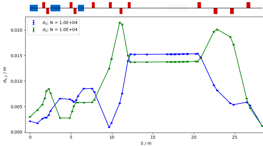
Figure 48: RMS beam size as a function of position along the beam line for a 127 MeV proton beam starting at the extraction line going through to the end of the in vivo beam line. The final four quadrupoles are matched in order to obtain \beta_{x,y} = 0.347 (blue).
