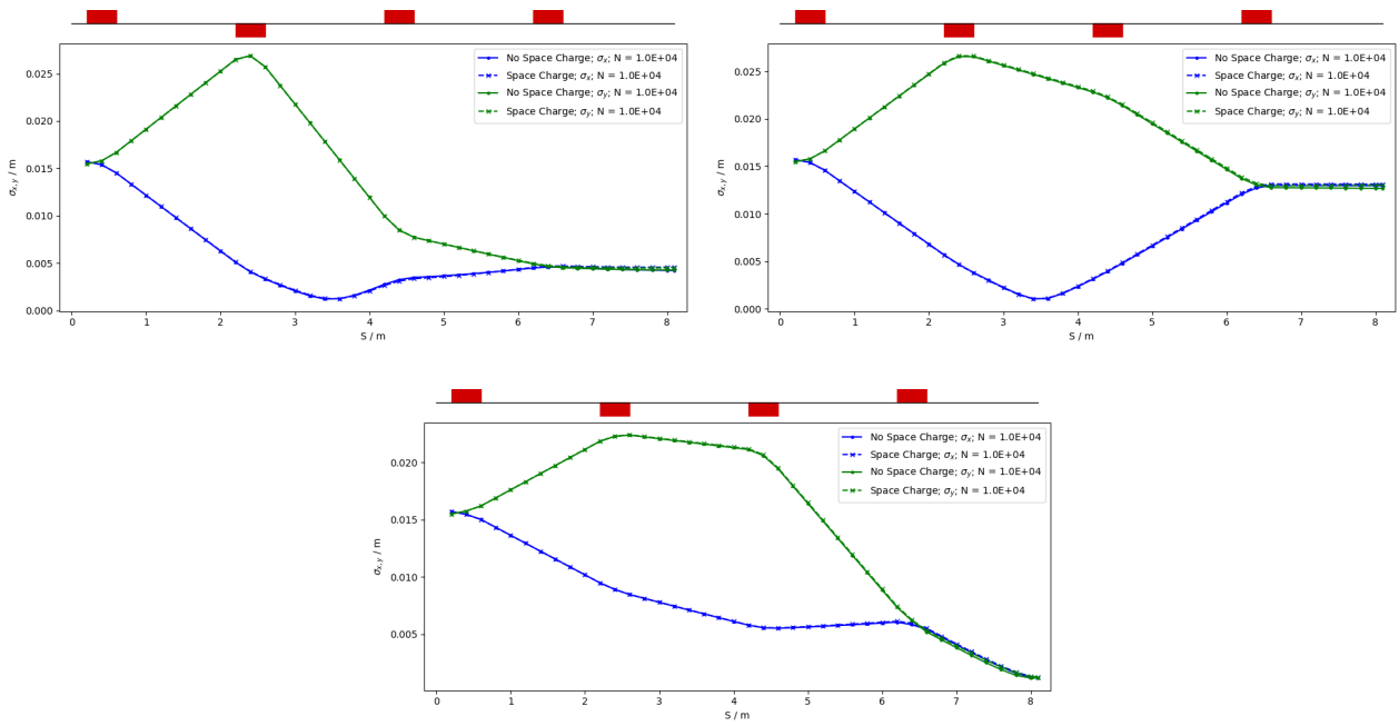
Figure 46: GPT simulations of the in vivo beamline for a 127 MeV proton beam with quadrupoles matched to \beta_{x,y} = 4.5 (upper left), \beta_{x,y} = 40 (upper right) and \beta_{x,y} = 0.347 (bottom) for 10^4 particles to investigate the effects of space charge. The solid line is when space charge is turned off, the dashed line when space charge is turned on.
