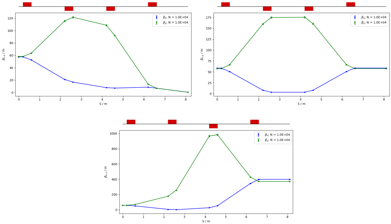
Figure 41: BDSIM simulations of the in vivo beamline for a 15 MeV proton beam with quadrupoles matched to \beta_{x,y} = 0.347 (upper left), \beta_{x,y} = 58 (upper right) and \beta_{x,y} = 395 (bottom) for 10^4 particles.
