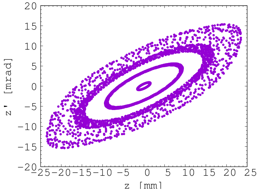
Figure 33: The results of the vertical dynamical acceptance study in the FFA ring. The 1 mm offset is assumed in the horizontal plane.
