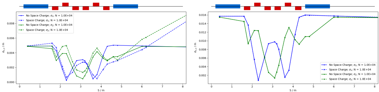
Figure 36: GPT simulation investigating the effects of space charge for a 15 MeV (left) and 127 MeV (right) proton beam passing through the high energy in vitro arc simulated with 10^4 particles. The solid lines are simulations without space charge and dashed lines with space charge.
