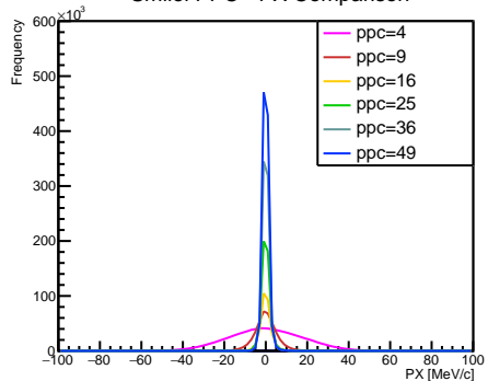
Smilei PPC - PX Comparison
