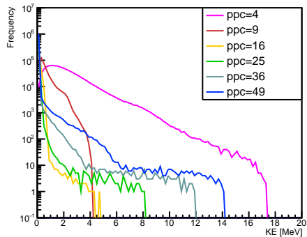
Smilei PPC - KE Comparison
