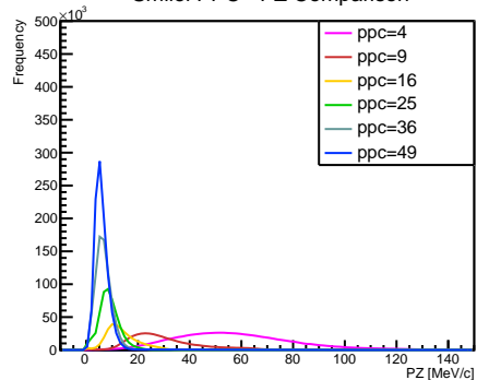
Smilei PPC - PZ Comparison
