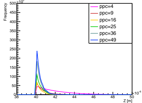
Smilei PPC - Z Comparison
