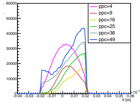
Smilei PPC - X Comparison
