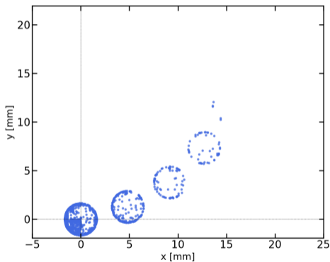
Generated macroparticles
