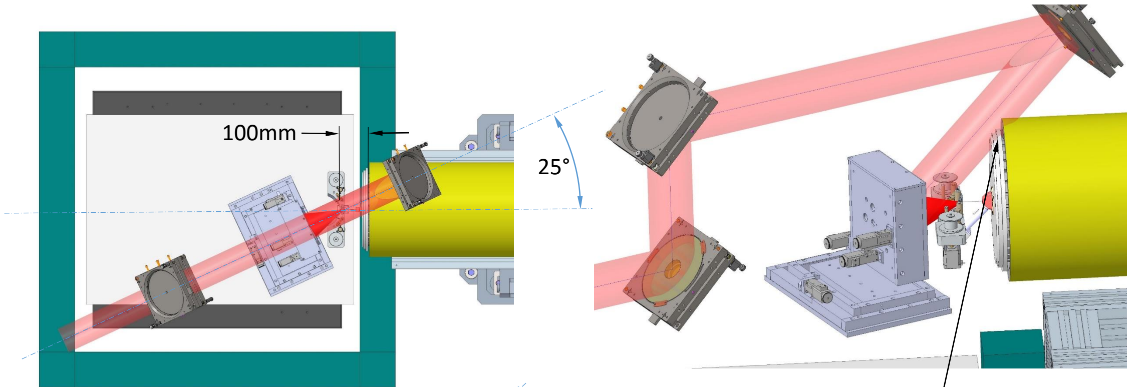
Plan View
